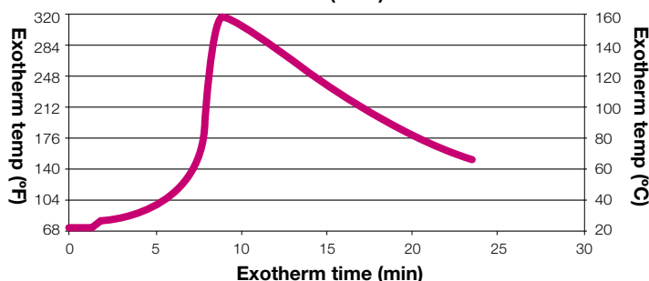
Typical Exotherm Curve for MA300 (10g mass) at 74°F (23°C) 5
